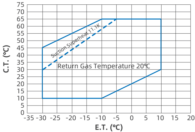
YIM38-72 R290
