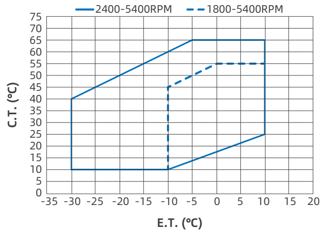
YIM38-72 R404A
