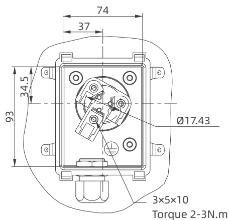
Wring diagram
