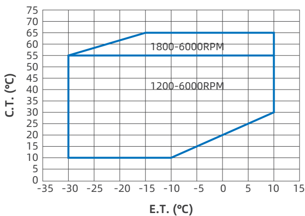
YIM38-72 R290
