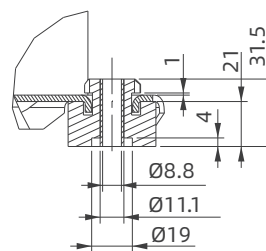
Mounting Feet
